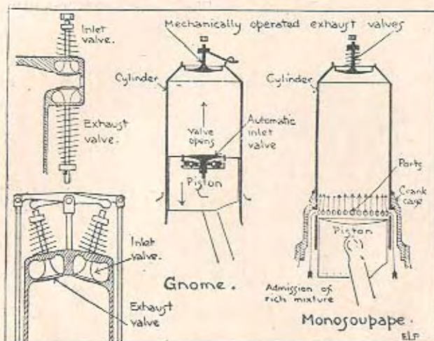
Arrangement of inlet and exhaust valves on aeroplane engines. Top left: The super-imposed arrangement. Bottom left: Overhead inlet and exhaust. Centre: Gnome pattern inlet in piston, and overhead exhaust. Right: Monosoupape or single-valve engine.
