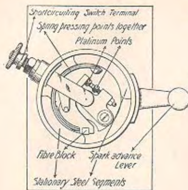
A complete magneto contact breaker (left), and details of the make and break (right).
