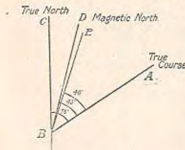
Indicating whether variation or deviation has to be added to or subtracted from the true course.
